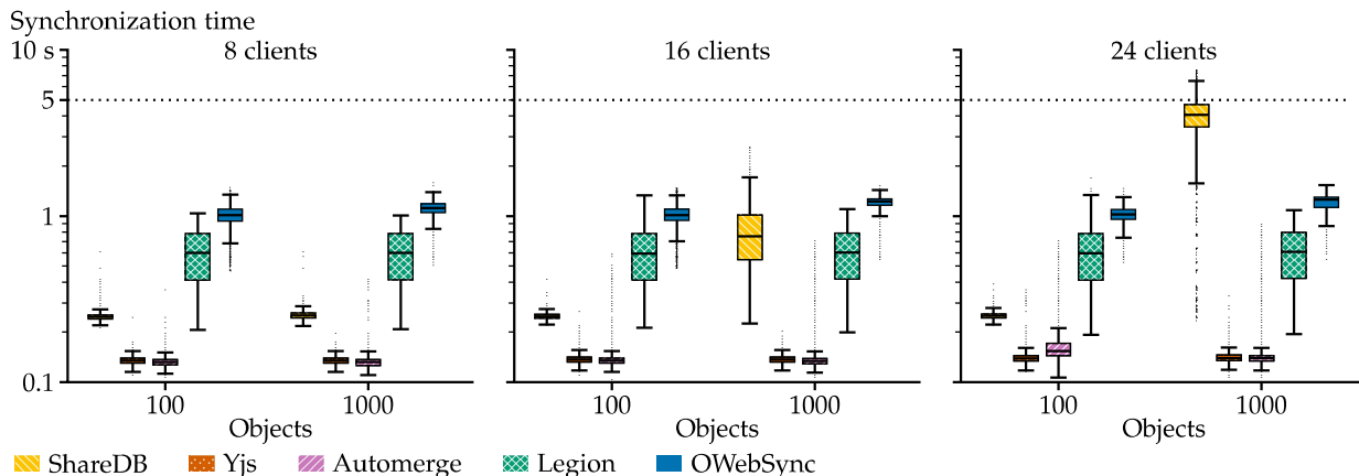
Fig. 6. Aggregated boxplots containing the times to achieve full synchronization to all clients in the online scenario. Each boxplot contains all 10 iterations for each of the 30 tests in the fully online situation. To compare technologies that have results of the same order of magnitude, as well as results in different orders of magnitude, we opted for a logarithmic Y-axis.
