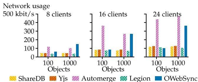
Fig. 7. Network usage per client for each test in the online scenario.
