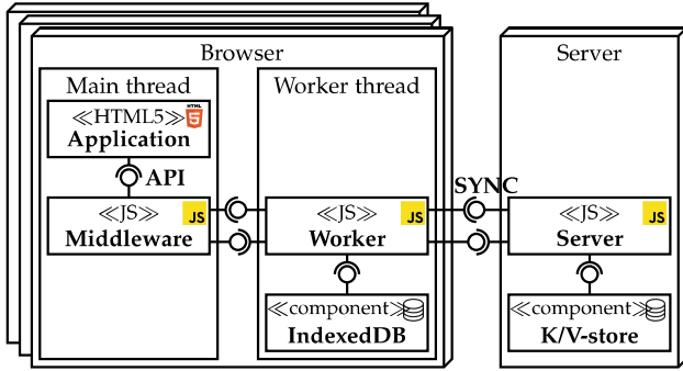
Fig. 4. Overall architecture of the OWebSync middleware
