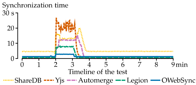
Fig. 9. Mean time to synchronize updates in case of a network disruption between minute 2 and 3 for the test with 24 clients, 1000 objects.
