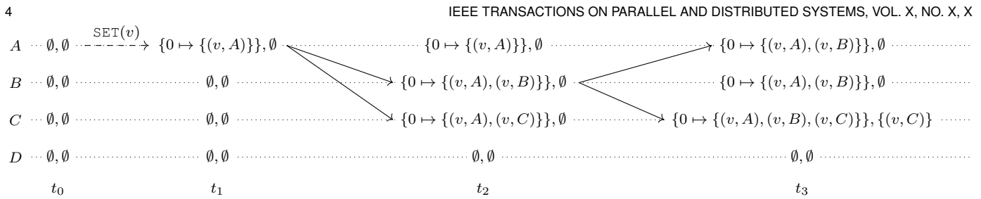
Fig. 2. Example of the state-based synchronization with 4 replicas A, B, C, D . Only the current votes and qc' are shown. Arrows represent a state transfer.
