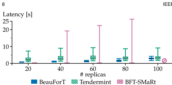
Fig. 7. Latency in the realistic scenario with network failures.
